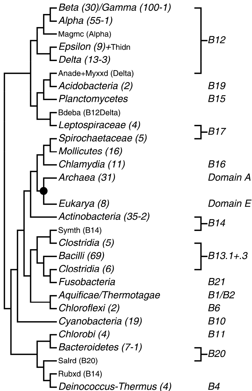
Fig. 1. The highest rank CVTree at K=5 . A taxon name represents a monophyletic cluster with the number of organisms given in parentheses. For example, Gamma(100-1) is the cluster of Gammaproteobacteria with 99 organisms, the “outlier” Thidn actually finds its correct placement in the Epsilon group. Outliers are given in smaller font. Given on the right are the phylum numbers in Bergey’s Outline Rel. 5 (Garrity et al., 2004). The black dot denotes the trifurcation point of the main domains of life. Note that this is an unrooted tree and the branches are not to scale.
